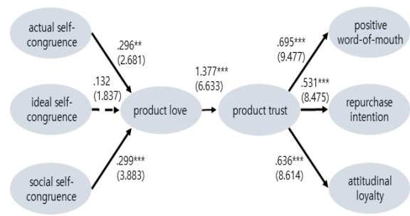
Figure 2. Estimates Final Structural Model
